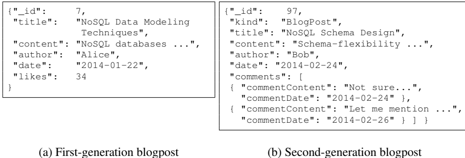
Figure 1: The structure of persisted JSON documents changes due to software- and schema evolution. Schema-free NoSQL data stores allow for heterogeneous documents to co-exist
