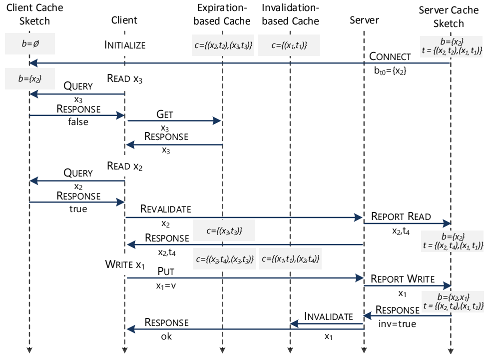
Figure 3: An end-to-end example of the proposed Cache Sketch methodology.
