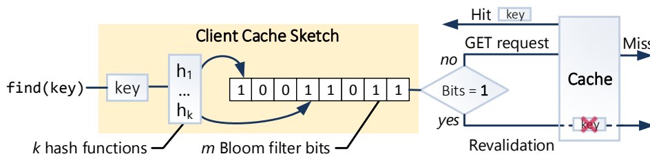
Figure 2: Database read using the Cache Sketch.
