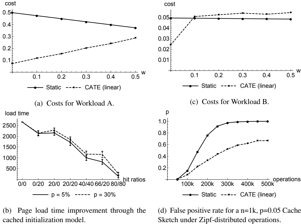
Figure 7: YMCA simulation results.
