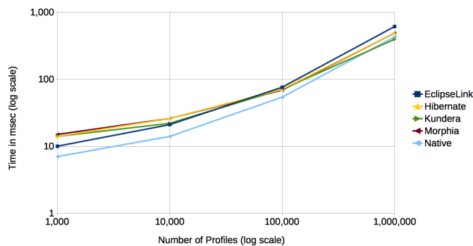
Figure 11: Scale up in evaluating Query 4 (MongoDB), not showing DataNucleus.
